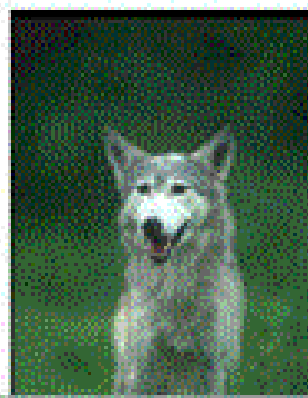
2: 110067 (score = 0.98)
