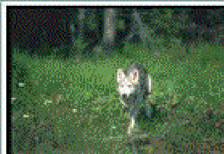
2: 110067 (score = 0.98)
