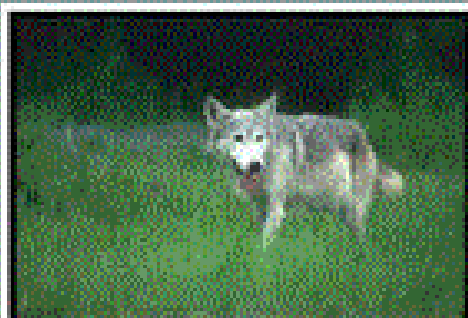
1: 110055 (score = 0.99)
